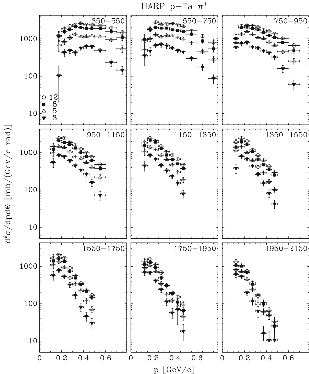
Fig. 23. Double-differential cross-sections for \pi^+ production in p -Ta interactions as a function of momentum displayed in different angular bins (shown in mrad in the panels). The results are given for all incident beam momenta ( filled triangles : 3 GeV/c; open triangles : 5 GeV/c; filled rectangles : 8 GeV/c; open circles : 12 GeV/c). The error bars take into account the correlations of the systematic uncertainties
