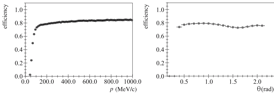
Fig. 16. Left: the efficiency as a function of total momentum at their production point for pions. Right: the efficiency as a function of \theta for pions
