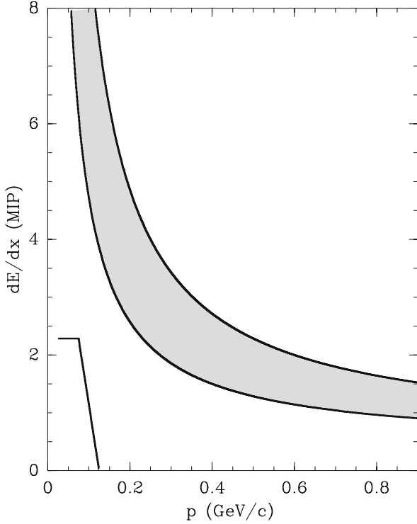
Fig. 20. Criteria used for the PID selection using the dE/dx (expressed in MIP) as a function of the measured momentum of the particle. Low momentum electrons and positrons are rejected when their dE/dx is below the lower left curve. The remaining particles are classified as protons if their dE/dx is above the gray band , as pions if they are below the gray band and rejected when they lie inside the gray band . The value of the MIP is calibrated for each setting
