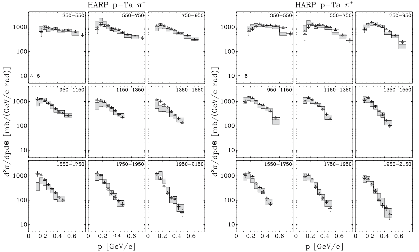
Fig. 31. Comparison of the double-differential cross-sections measured for \pi^+ (right) and \pi^- (left) production in p -Ta interactions as a function of momentum displayed in different angular bins using the two analyses. The results of the alternative analysis are shown as shaded band and are available only for 5 GeV/c incident beam momentum. The width of the band represents an estimate of the uncorrelated error (one standard deviation) between the two methods. The results of the standard analysis described in this paper are represented by data points
