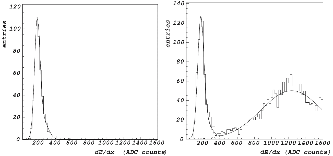
Fig. 18. dE/dx spectra for negative particles (on the left) and positive (on the right) with momentum between 300 MeV/c and 350 MeV/c. The curves show the Landau distributions fitted to the data. The protons are clearly visible in the distribution for positive particles at high dE/dx and absent for the negatively charged particles
