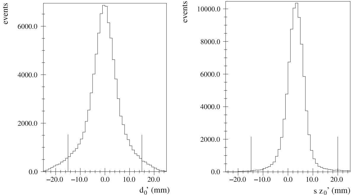
Fig. 7. The distribution of d'_0 (left panel) and sz'_0 (right panel) taken with an 8 GeV/c proton beam hitting a tantalum target for tracks with low dE/dx . Cuts (indicated by the vertical bars) are applied at |d'_0| < 15 mm and -14.4 mm < sz'_0 < 20.0 mm
