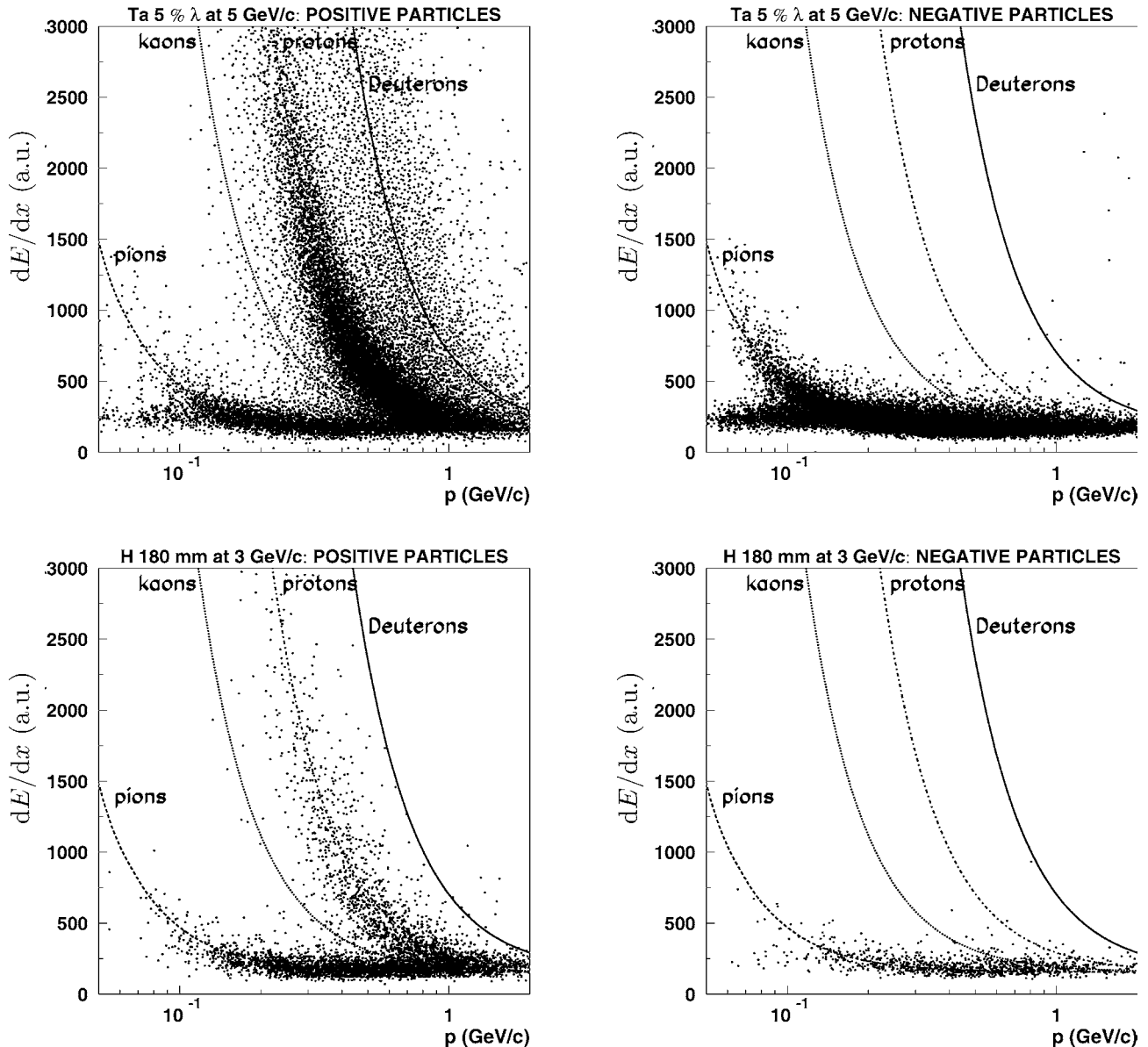
Fig. 17. dE/dx (in arbitrary units) versus momentum (in GeV/c). Top: p -tantalum data in the 5 GeV/c beam; Bottom: p -hydrogen data in the 3 GeV/c beam; Left: for positive tracks; Right: for negative tracks. The lines are simple \beta^{-2} curves and merely indicate the regions populated by the various particle types. The fact that the band marked 'deuterons' is not present in the hydrogen data clearly shows that the population in this band in the tantalum data is not an artefact of the momentum reconstruction but deuteron production
