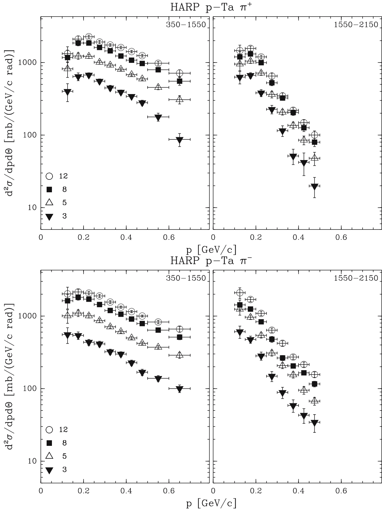
Fig. 26. Double-differential cross-sections for \pi^+ ( top panel ) and \pi^- ( bottom panel ) production in p -Ta interactions as a function of momentum averaged over the angular region covered by this experiment (shown in mrad). Left: forward production ( 350 \text{ mrad} \leq \theta < 1550 \text{ mrad} ); Right: backward production ( 1550 \text{ mrad} \leq \theta < 2150 \text{ mrad} ). The results are given for all incident beam momenta ( filled triangles: 3 \text{GeV}/c ; open triangles: 5 \text{GeV}/c ; filled rectangles: 8 \text{GeV}/c ; open circles: 12 \text{GeV}/c )
