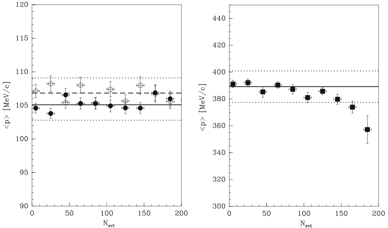
Fig. 15. Comparison of the average reconstructed momentum as a function of event number in spill: left, for charged pions selected using dE/dx , open circles are for \pi^- , closed circles are for \pi^+ ; right, for protons using a higher value of dE/dx for the selection. In the left panel the straight lines indicate the average values for the first 100 events: dashed line for \pi^- and solid line for \pi^+ . In the right plot the solid line shows the average for protons for the first 100 events. The dotted lines in both panels show the \pm 3\% variation around the averages. For both panels a selection 1.0 \text{ rad} < \theta < 1.5 \text{ rad} was applied to ensure a limited range of p_T . For the protons in the right panel the requirement that they have a hit in both barrel RPC layers was applied to set a momentum threshold
