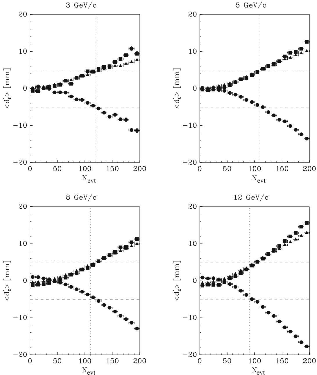
Fig. 4. Effect of dynamic distortions as a function of event number in the spill for the four tantalum settings used in the analysis emphasizing the first part of the spill (200 events). The symbols show the average extrapolated distance from the incoming beam particle trajectory for \pi^- (filled circles), \pi^+ (filled squares), and protons (filled triangles). The momentum of the beam is indicated in the title of the panels. Data with \langle d'_0 \rangle < 5 mm have been used in the analysis. The dashed horizontal lines indicate the value at \pm 5 mm to guide the eye, while the vertical dotted lines show the maximum value of N_{\text{evt}} accepted in the analysis
