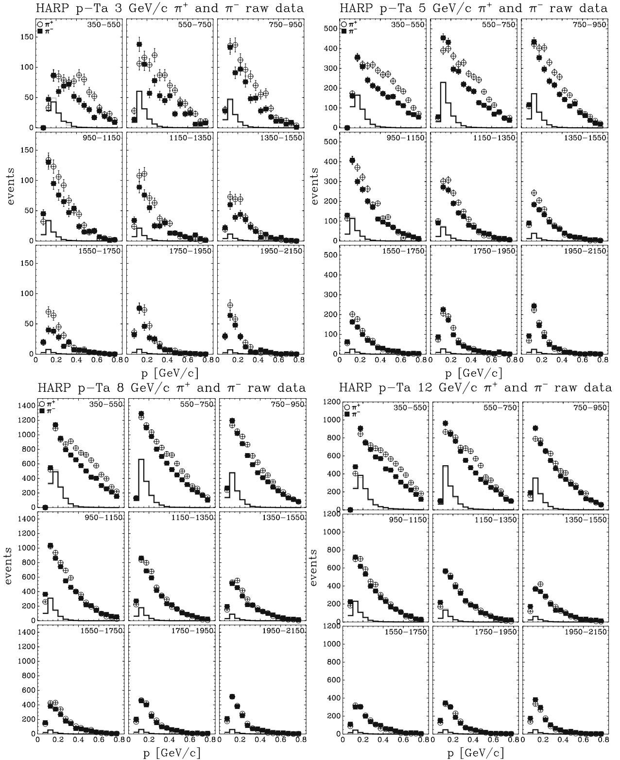
Fig. 22. Distribution for positive ( open circles ) and negative pions ( filled squares ) using the PID algorithm based on dE/dx as a function of momentum and in different angular bins (indicated in mrad in the panels) taken with 3 GeV/c, 5 GeV/c, 8 GeV/c and 12 GeV/c proton beam hitting a tantalum target. The histograms show the distributions calculated for the \pi^0 subtraction (see Sect. 6). The shaded (black) lines show the positrons (electrons) to be subtracted from the \pi^+ ( \pi^- ) spectra. The two sets of lines coincide almost everywhere as expected from the production mechanism and are therefore almost indistinguishable in the figure
