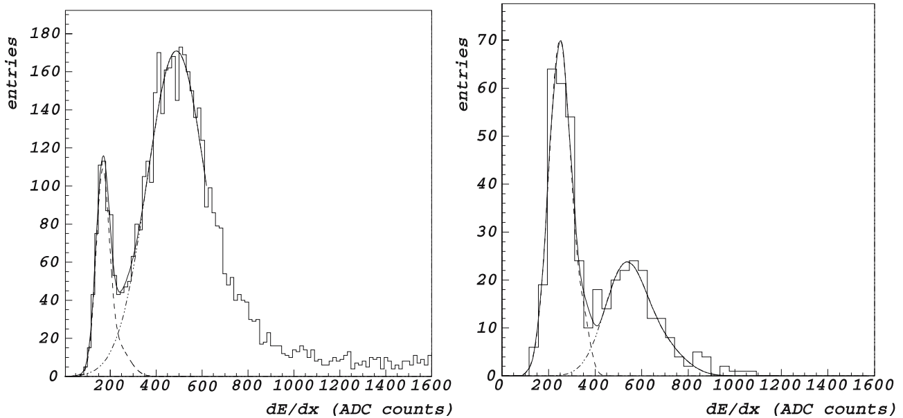
Fig. 19. Left panel: dE/dx spectra for positive particles with momentum between 500 MeV/c and 600 MeV/c. The curves show the Landau distributions fitted to the data. The distributions of pions and protons are distinct but not clearly separated. Right panel: The dE/dx spectrum for negative particles with momentum between 75 MeV/c and 100 MeV/c. The curves indicate the fits to the two components using two Landau distributions. The distribution of the electrons with low dE/dx is clearly visible to the left of the highly ionizing negative pions
