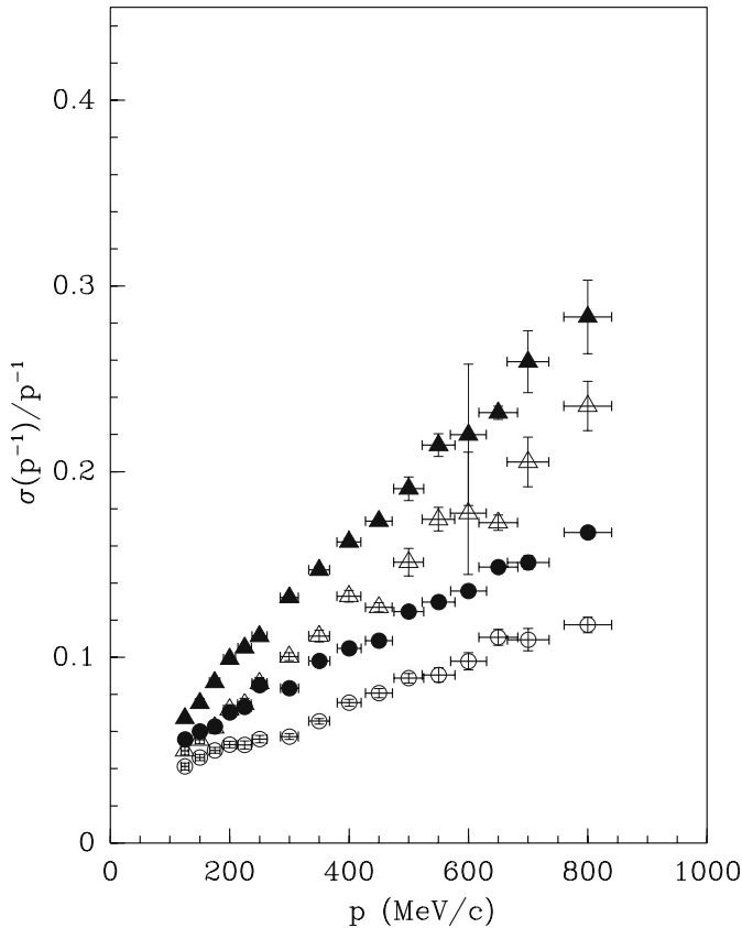
Fig. 5. Simulation study of the resolution of the inverse of the momentum determination using the constraint of the extrapolated beam particle. Results for charged pions emitted at large angles ( 85^\circ ) are shown with triangles, while the circles represent the behaviour at smaller angles ( 35^\circ ). The resolution of the measured momentum is compared with the ‘true’ momentum in the gas. All materials in the detector and the target are taken into account in the simulation. A fit with two Gaussians constrained to have the same mean has been performed to the distributions. Filled circles and triangles show the measurement of the RMS of the fitted function, while the open circles and triangles show the \sigma of the narrow Gaussian
