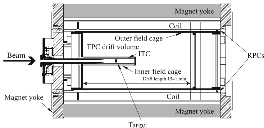
Fig. 3. Schematic layout of the TPC. The beam enters from the left. Starting from the outside, first the return yoke of the magnet is seen, closed with an end-cap at the upstream end, and open at the downstream end. The cylindrical coils are drawn inside the yoke. The field cage is positioned inside this magnetic volume. The inner field cage is visible as a short cylinder entering from the left. The ITC trigger counter and the target holder are inserted in the inner field cage. The RPCs (not drawn) are positioned between the outer field cage and the coil
