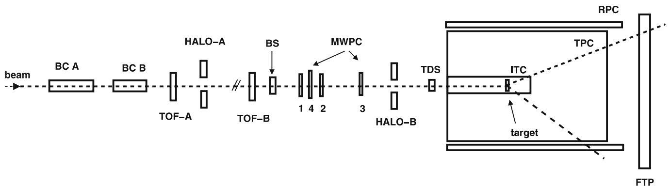
Fig. 2. Schematic view of the trigger and beam equipment. The description is given in the text. The beam enters from the left. The MWPCs are numbered: 1, 4, 2, 3 from left to right. On the right, the position of the target inside the inner field cage of the TPC is shown
