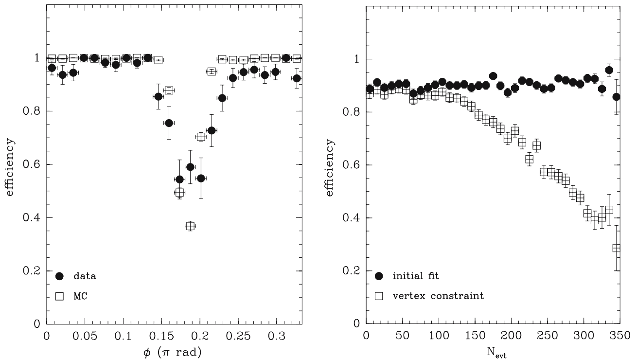
Fig. 10. Left panel: the track finding efficiency as a function of \phi within the sectors of the pad-plane of the TPC for 8 GeV/c elastic scattering data measured with elastic events (first 80 events in the spill). The filled circles show the efficiency for recognizing tracks including the fit to a helix in the data, the open squares show the simulated efficiency. The integral of the efficiency is well reproduced, although the details near the spokes are different. Right panel: Efficiency for the pattern recognition and momentum reconstruction for elastically produced recoil protons as a function of event number in spill. Closed circles: trajectory fit without vertex constraint; open squares: trajectory fit with vertex constraint. The efficiency includes the effect of the cut on d'_0 . The efficiency for the reconstruction and fit using the vertex constraint remains constant within \approx 1\% up to a distortion corresponding to \langle d'_0 \rangle = 6 mm
