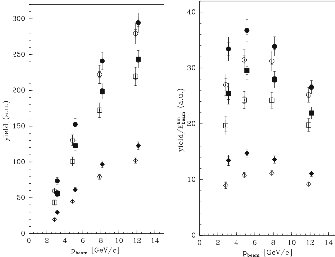
Fig. 30. Prediction of the \pi^+ (closed symbols) and \pi^- (open symbols) yield as a function of incident proton beam momentum for different designs of the neutrino factory focusing stage. Shown are the integrated yields (left) and the integrated yields normalized to the kinetic energy of the proton (right). The circles indicate the integral over the full HARP acceptance, the squares are integrated over 0.35 \text{ rad} < \theta < 0.95 \text{ rad} , while the diamonds are calculated for the restricted angular range and 250 \text{ MeV}/c < p < 500 \text{ MeV}/c . The full error bar shows the overall (systematic and statistical) error, while the inner error bar shows the error relevant for the point-to-point comparison. For the latter error only the uncorrelated systematic uncertainties were added to the statistical error
