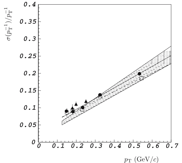
Fig. 9. Momentum resolution in the TPC. The filled circles ( open boxes ) and the drawn (dashed) straight line refer to the cosmic-ray data taken in 2003 (2002). The filled triangles are the upper limits ('over-estimates') obtained from the dE/dx selection. The shaded area refers to a straight-line fit to the Monte Carlo calculations
