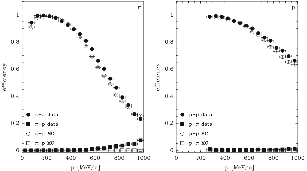
Fig. 21. Performance of the PID using the dE/dx as a function of the measured momentum of the particle. The particles are selected using TOF. Left: for negative pions produced in a positive pion beam; Right: for protons produced in a proton beam. The filled (open) circles show the efficiency measured with the data (Monte Carlo), the filled (open) squares represent the fraction of particles misidentified as anti-protons ( left ) and pions ( right ) in the data (Monte Carlo)
