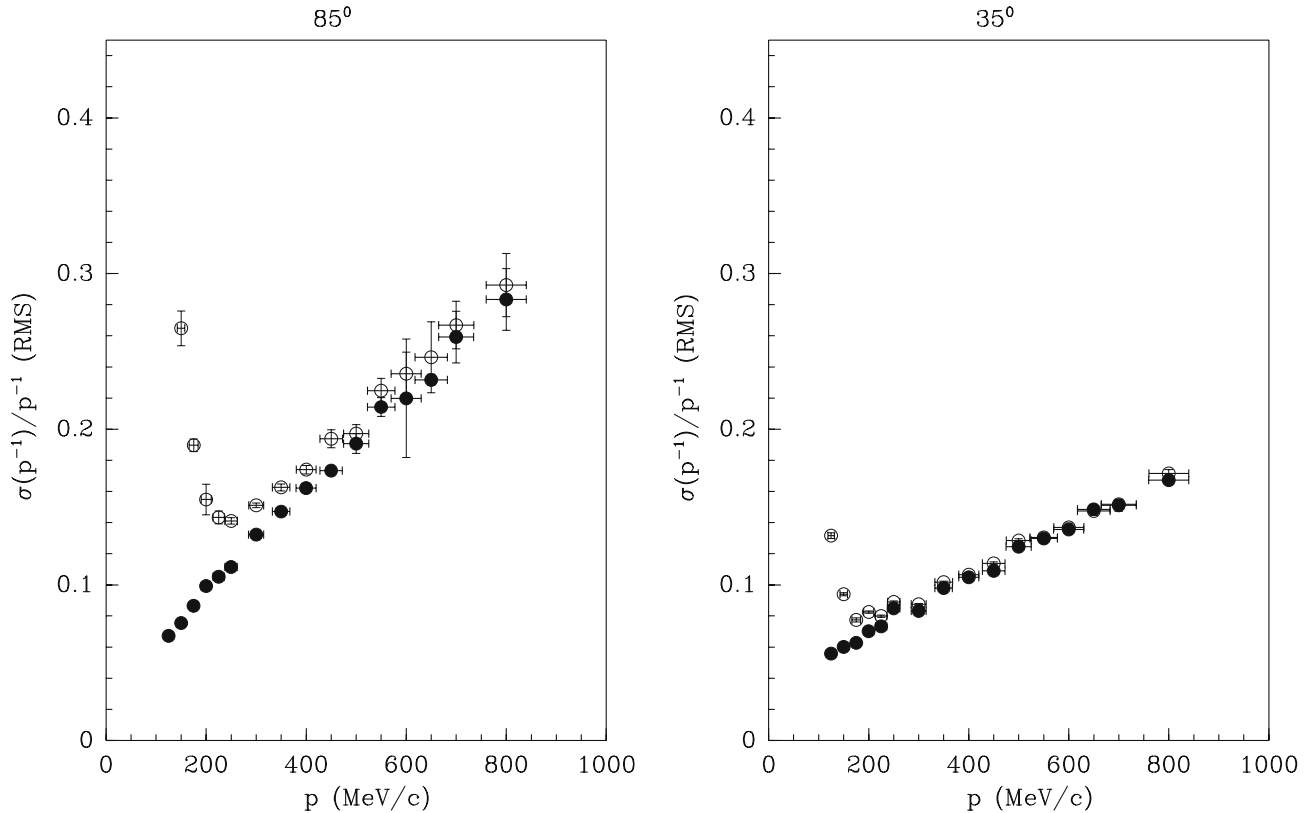
Fig. 6. Simulation study of the resolution of the determination of the inverse of the momentum using the constraint of the extrapolated beam particle. The left panel shows the results for charged pions emitted at large angles ( 85^\circ ), while the right panel shows the behaviour at smaller angles ( 35^\circ ). All materials in the detector and the target are taken into account. Filled circles show the resolution of the inverse of the momentum determination with respect to the ‘true’ momentum of the particle in the TPC gas volume for pions (measured by the RMS of the distribution). Open circles and boxes show the resolution with respect to the ‘true’ momentum at the interaction vertex. The effect of energy-loss in the material (target, trigger detector, IFC) is clearly visible
