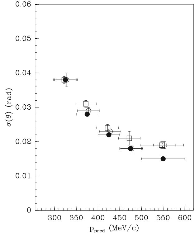
Fig. 12. The resolution in \theta for elastic scattering (3 GeV/ c : open boxes, 5 GeV/ c : open circles) data measured with elastic events as a function of the momentum predicted by the forward scattered track compared to a simulation of the same sample of events at 5 GeV/ c (filled circles)
