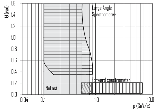
Fig. 29. Kinematic region in the p - \theta plane covered by this analysis compared to the maximum acceptance of an input stage of typical neutrino factory designs. The different neutrino factory designs have in addition to the limits shown different limits in p_T
