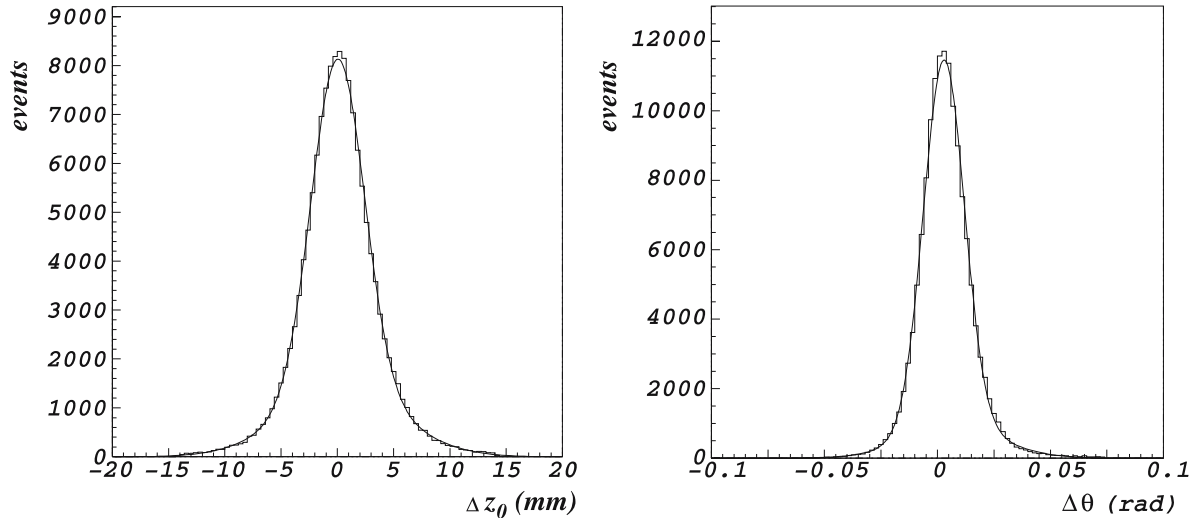
Fig. 8. Left: Measurement with cosmic-ray tracks of the z'_0 resolution of the TPC. The distribution has an RMS of 3.4 mm. Right: measurement with cosmic-ray tracks of the \theta resolution of the TPC. The distribution has an RMS of 12 mrad
