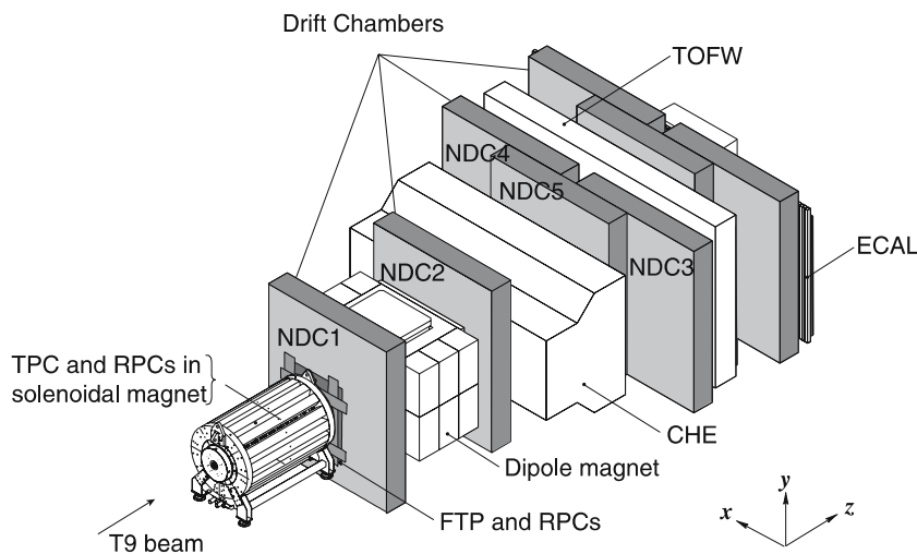
Fig. 1. Schematic layout of the HARP detector. The convention for the coordinate system is shown in the lower-right corner . The three most downstream (unlabelled) drift chamber modules are only partly equipped with electronics and are not used for tracking. The detector covers a total length of 13.5 m along the beam direction and has a maximum width of 6.5 m perpendicular to the beam
