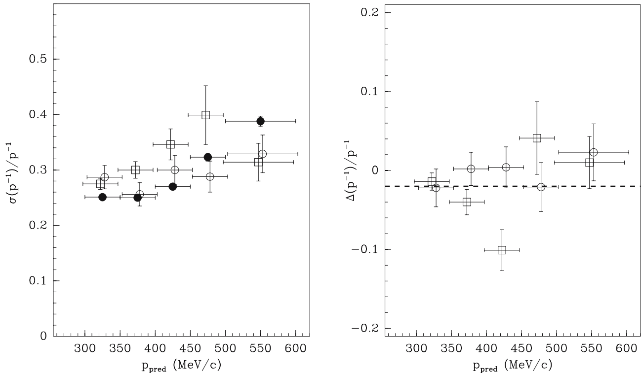
Fig. 13. Left panel: The momentum resolution of the fit without vertex constraint for elastic scattering data (3 GeV/c: open squares, 5 GeV/c: open circles) measured with elastic events as a function of the momentum predicted by the forward scattered track. The resolution is dominated by the effect of energy-loss and multiple scattering and is consistent with the measurement with cosmic-ray tracks. The filled circles show a full simulation of the elastic events using a realistic elastic cross-section model and detector description. The agreement between data and simulation is good. Right panel: the momentum bias of the fit without vertex constraint measured with elastic scattering data (3 GeV/c: open squares, 5 GeV/c: open circles) with elastic events as a function of the momentum predicted by the forward scattered track. In the absence of a clear trend, the average of the points constrains the bias to be smaller than 3%. For these comparisons only the first 50 events in the spill are used since the unconstrained fit is sensitive to dynamic distortions beyond this value
