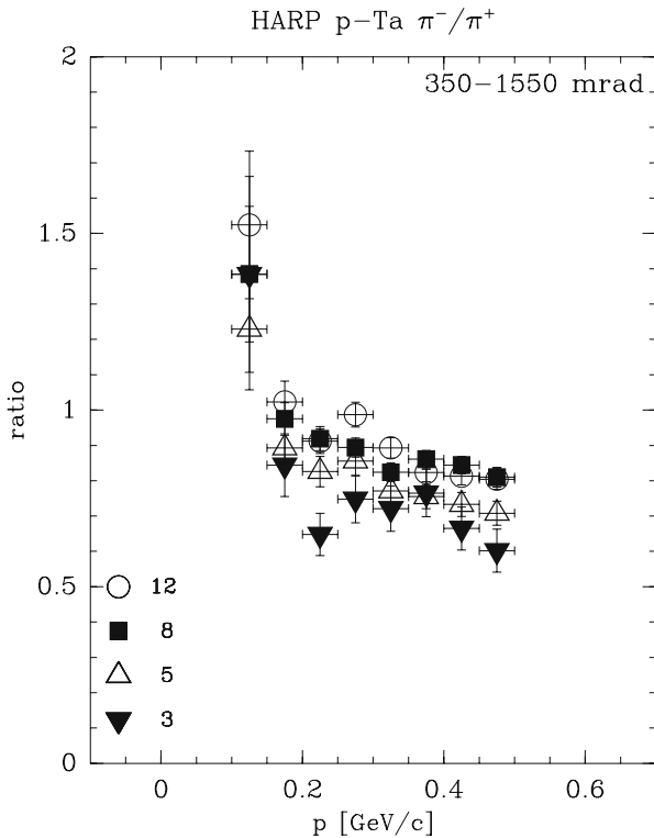
Fig. 27. The ratio of the differential cross-sections for \pi^- and \pi^+ production in p -Ta interactions as a function of momentum integrated over the forward angular region (shown in mrad). The results are given for all incident beam momenta ( filled triangles : 3 GeV/c; open triangles : 5 GeV/c; filled rectangles : 8 GeV/c; open circles : 12 GeV/c)
