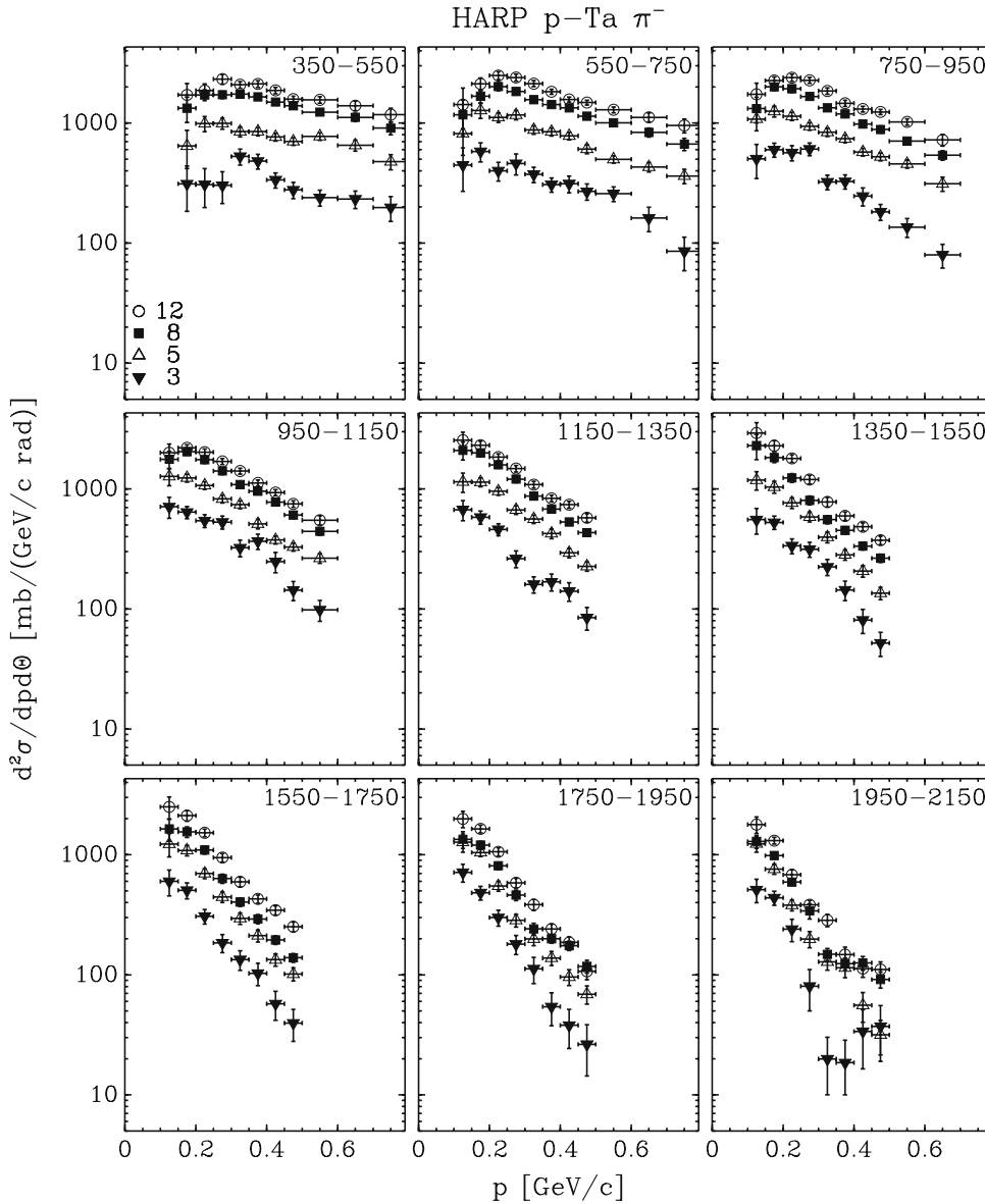
Fig. 24. Double-differential cross-sections for \pi^- production in p -Ta interactions as a function of momentum displayed in different angular bins (shown in mrad in the panels). The results are given for all incident beam momenta ( filled triangles : 3 GeV/c; open triangles : 5 GeV/c; filled rectangles : 8 GeV/c; open circles : 12 GeV/c). The error bars take into account the correlations of the systematic uncertainties
