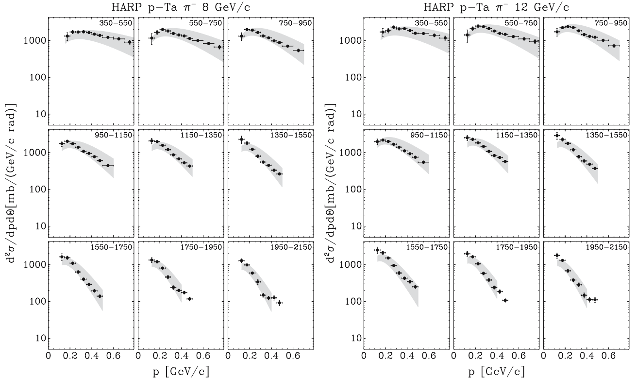
Fig. 28. Comparison of the HARP data with data from [41]. The left panel shows the comparison of the parametrization of the 10 GeV/c data of [41] with the 8 GeV/c data reported here; the right panel shows the comparison with the 12 GeV/c data. The absolute normalization of the parametrization was fixed to the data in both cases. The band shows the range allowed by varying the slope parameters given by [41] with two standard deviation and a 10% variation on the absolute scale
