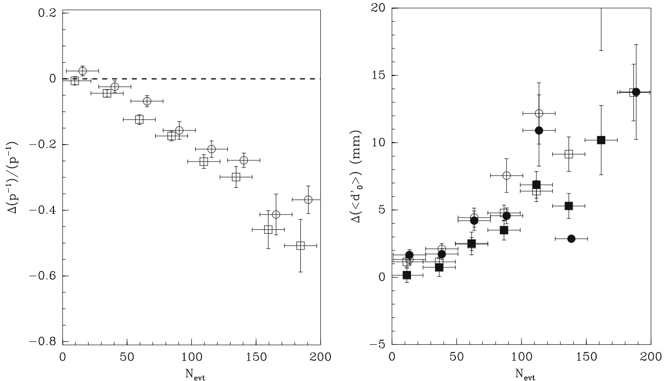
Fig. 11. Left panel: The shift in average momentum for elastic scattering data (3 GeV/c: open squares, 5 GeV/c: open circles) measured with elastic events as a function of the value of N_{\text{evt}} . The momentum estimator from the fit not constrained by the impact point of the incoming beam particle is used here. Right panel: The shift in average d'_0 as a function of the event number in spill for elastic scattering data (3 GeV/c: filled and open boxes, 5 GeV/c: filled and open circles) measured with elastic events as a function of the value of N_{\text{evt}} . The open symbols show the data for predicted momenta below 450 MeV/c and the filled symbols for predicted momenta above 450 MeV/c
