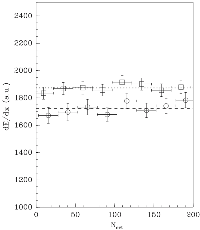
Fig. 14. The average value of dE/dx as a function of the event number in spill for elastic scattering data (3 GeV/c: open boxes, 5 GeV/c: open circles) measured with elastic events. The dotted and dashed lines show the average value for 3 GeV/c and 5 GeV/c, respectively
